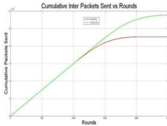
Figure 17: Overall Cumulative inter-cluster Packets vs Rounds
