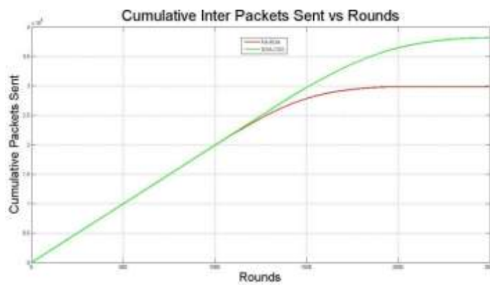
Figure 11: Overall Cumulative inter-cluster Packets vs Rounds
