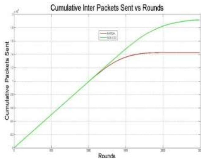
Figure 5: Overall Cumulative inter-cluster Packets vs Rounds
