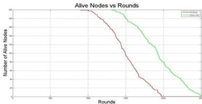
Figure 8: Alive Nodes vs Rounds
