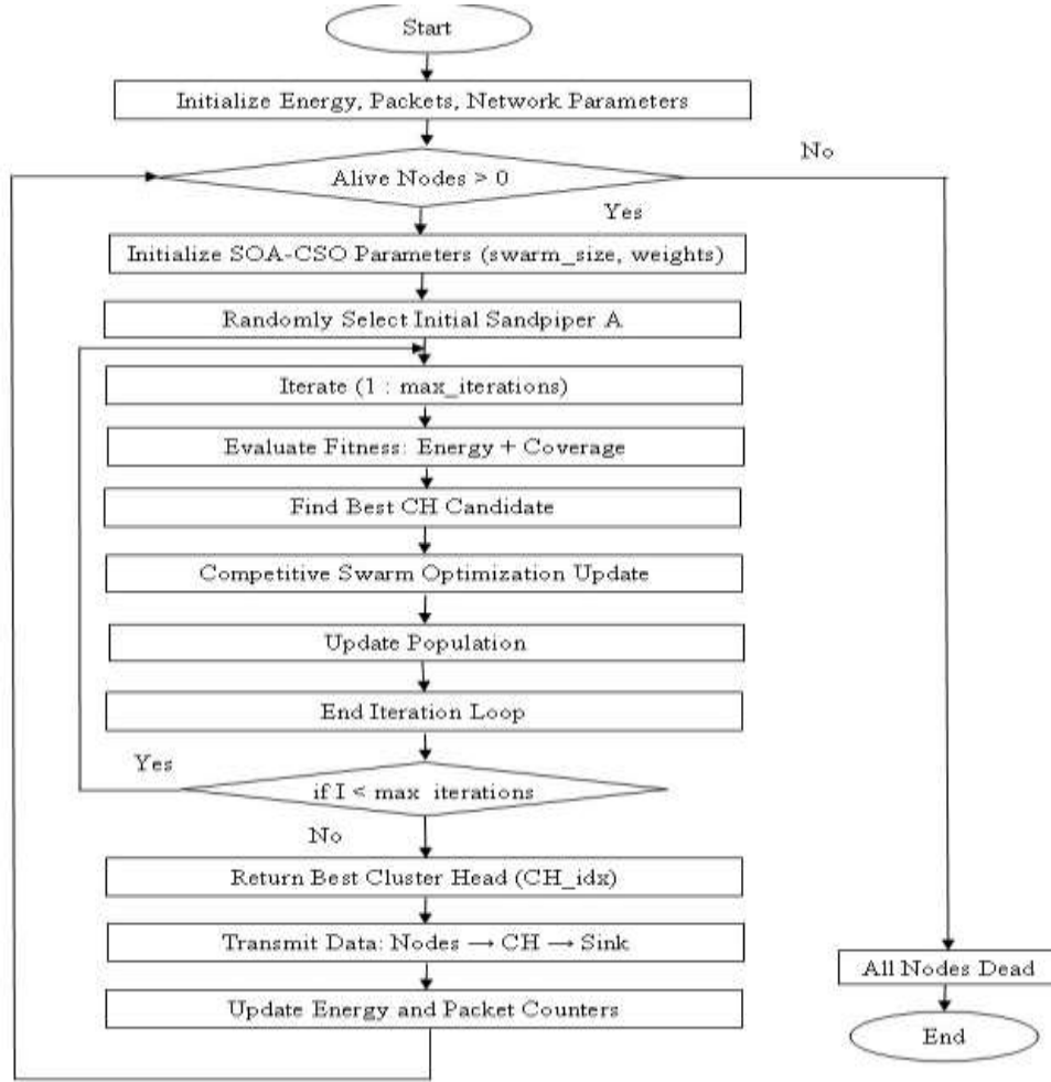
Figure 1: Flowchart of the proposed Hybrid SOA-CSO Cluster Head Selection
